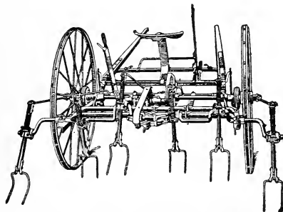
HAY TEDDER, McCORMICK-DEERING
